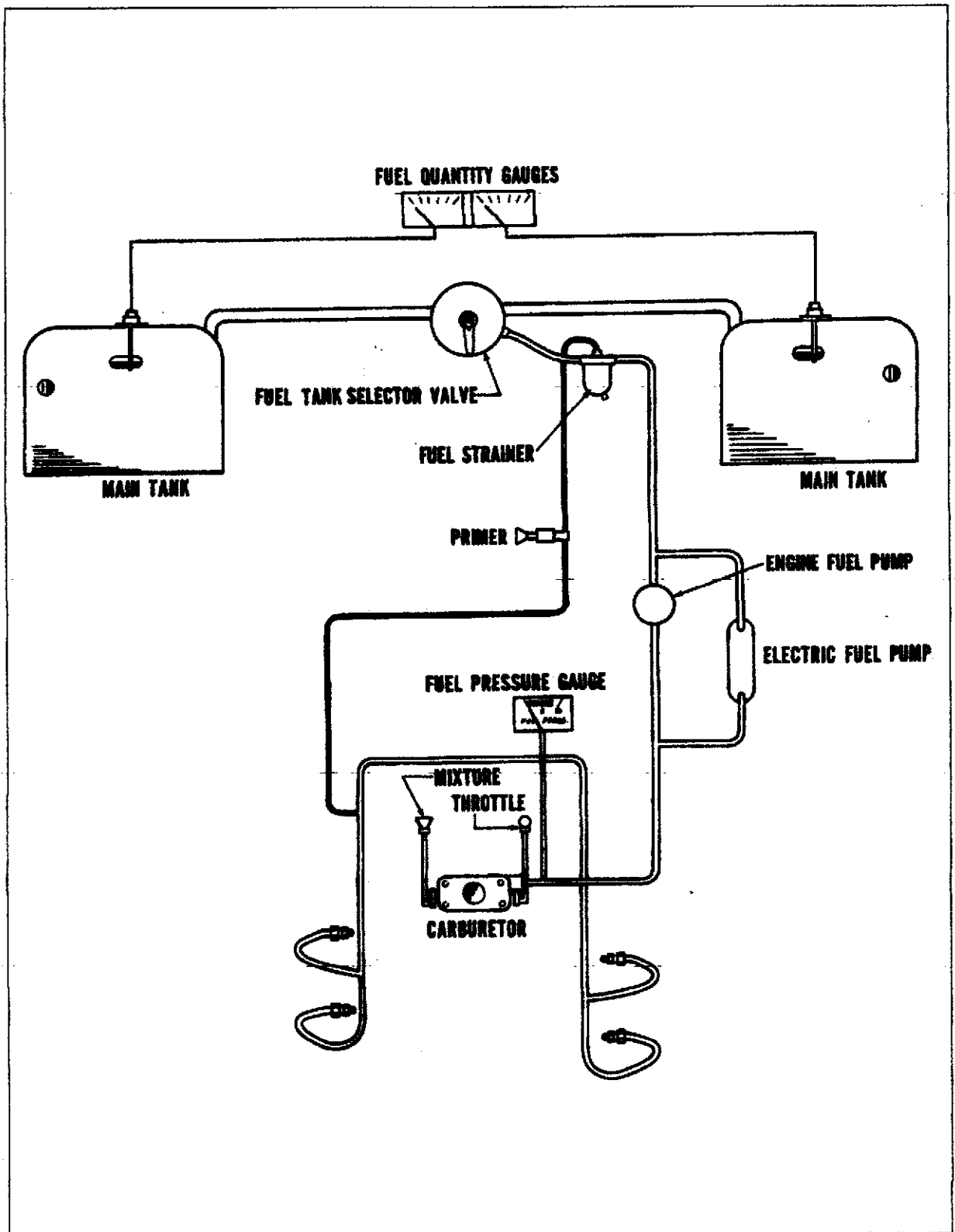
Fuel System Schematic
