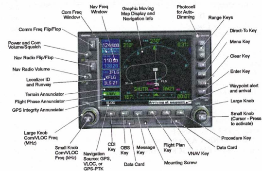
Figure 1 - 500W Series Control and Display Layout
