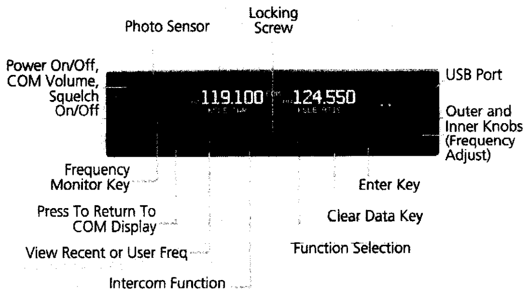
GTR 225 Front Panel Description
