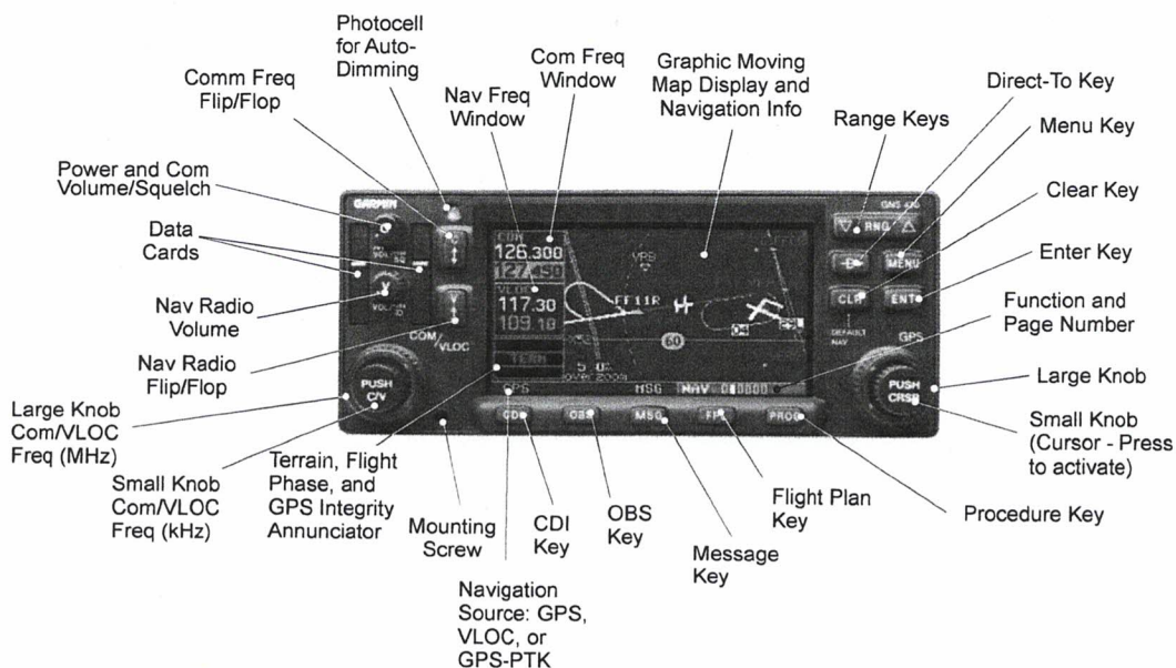
Figure 1 - 430W Series Control and Display Layout
